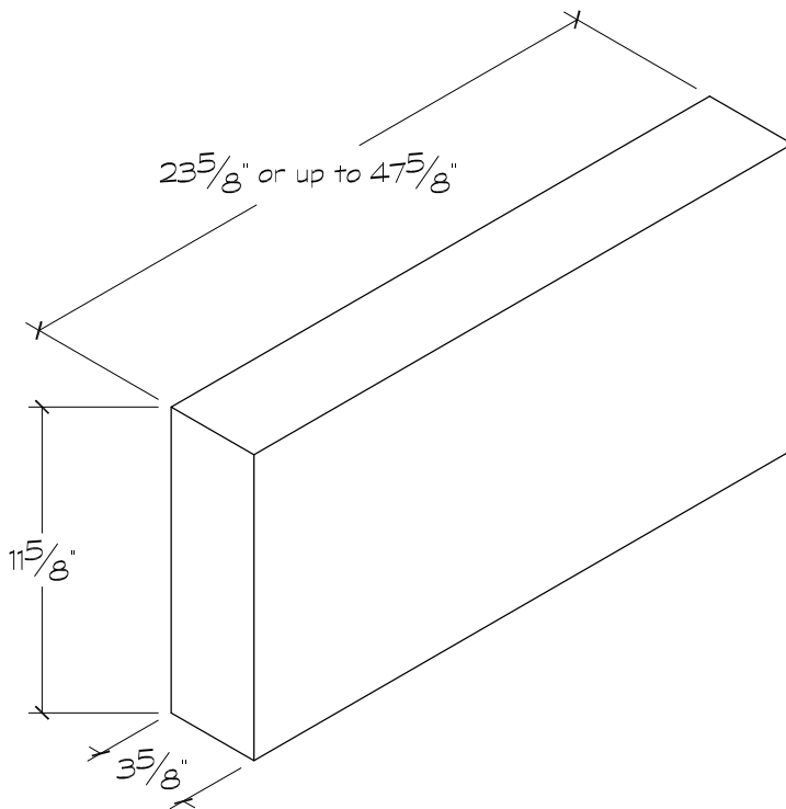
ISO VIEW
